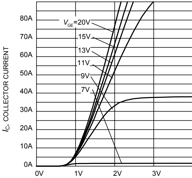
Figure 5. Typical output characteristic ( T_j = 25^\circ\text{C} )
