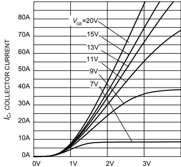
Figure 6. Typical output characteristic ( T_j = 175^\circ\text{C} )
