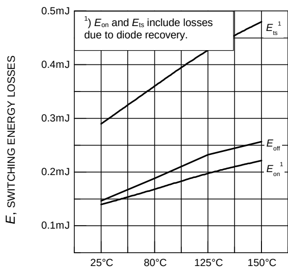
Figure 15. Typical switching energy losses as a function of junction temperature (inductive load, V_{CE} = 800\text{V} , V_{GE} = +15\text{V}/0\text{V} , I_C = 3\text{A} , R_G = 82\Omega , dynamic test circuit in Fig.E )
