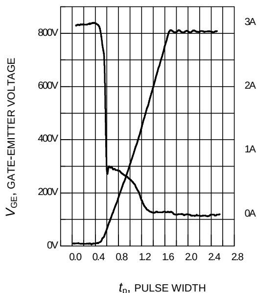
Figure 21. Typical turn off behavior, soft switching ( V_{GE}=15/0V , R_G=82\Omega , T_j=150^\circ C , Dynamic test circuit in Figure E)
