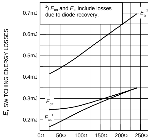
Figure 14. Typical switching energy losses as a function of gate resistor (inductive load, T_j = 150^\circ\text{C} , V_{CE} = 800\text{V} , V_{GE} = +15\text{V}/0\text{V} , I_C = 3\text{A} , dynamic test circuit in Fig.E )
