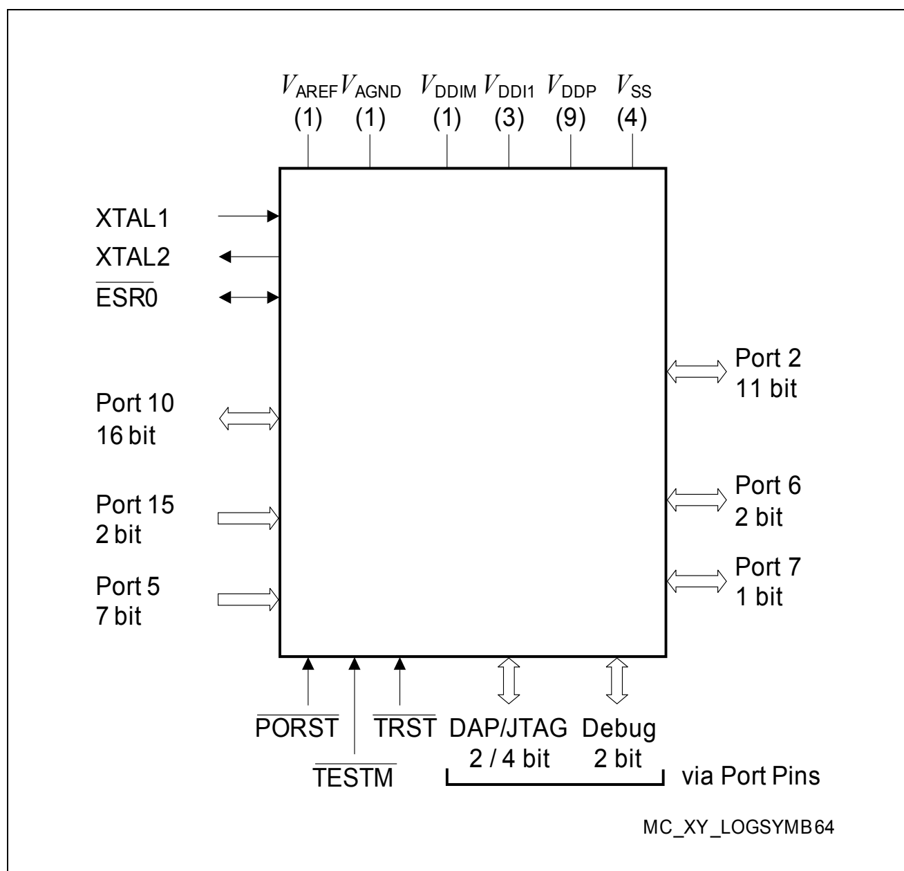
Figure 2 XC223xN Logic Symbol
