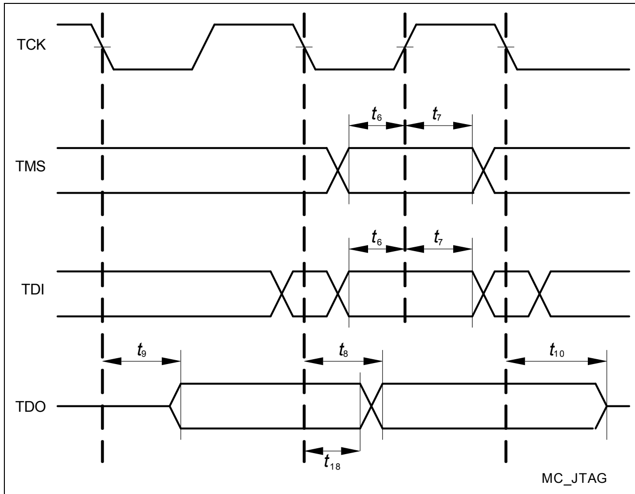
Figure 27 JTAG Timing
