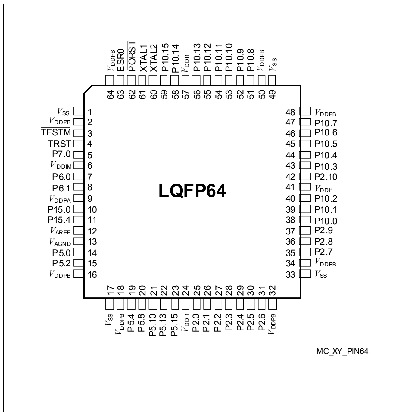
Figure 3 XC223xN Pin Configuration (top view)
