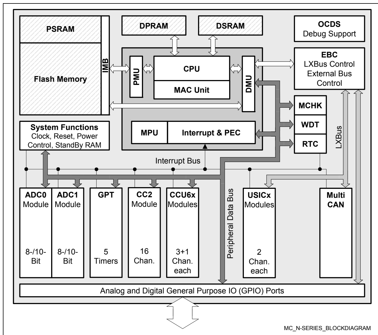
Figure 4 Block Diagram
