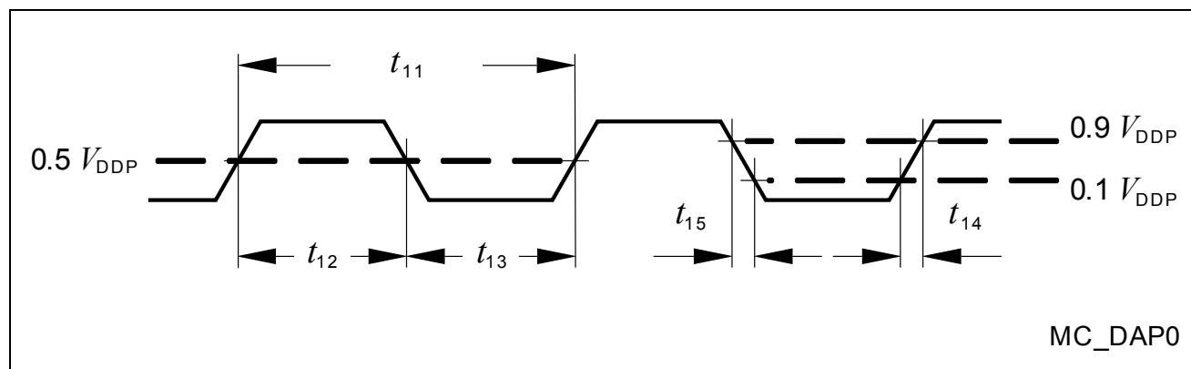
Figure 23 Test Clock Timing (DAP0)
