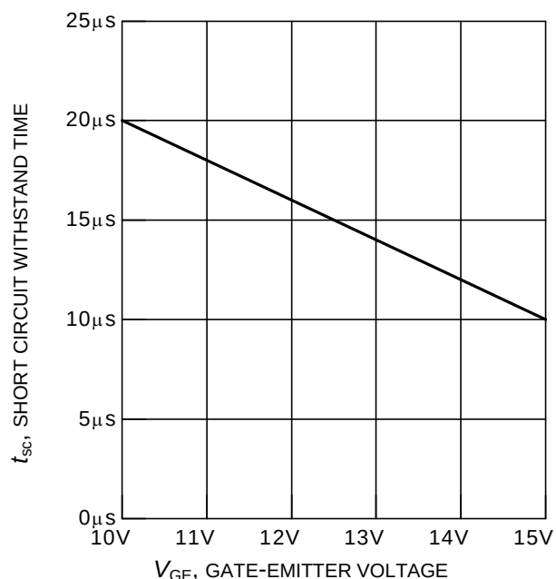
Figure 19. Short circuit withstand time as a function of gate-emitter voltage ( V_{CE} = 600V , start at T_i = 25^\circ C )
