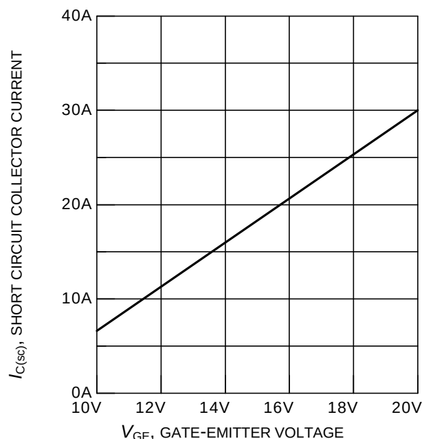
Figure 20. Typical short circuit collector current as a function of gate-emitter voltage ( V_{CE} \leq 600V, T_i = 150^\circ C )
