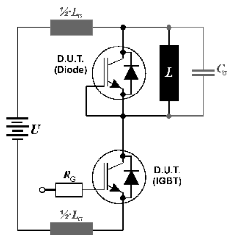
Figure E. Dynamic test circuit Leakage inductance L_{\sigma} =180nH and Stray capacity C_{\sigma} =180pF.
