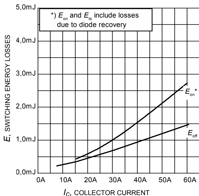
Figure 13. Typical switching energy losses as a function of collector current (inductive load, T_J=150^{\circ}\text{C} , V_{CE}=400\text{V} , V_{GE}=0/15\text{V} , R_G=11\Omega , Dynamic test circuit in Figure E)
