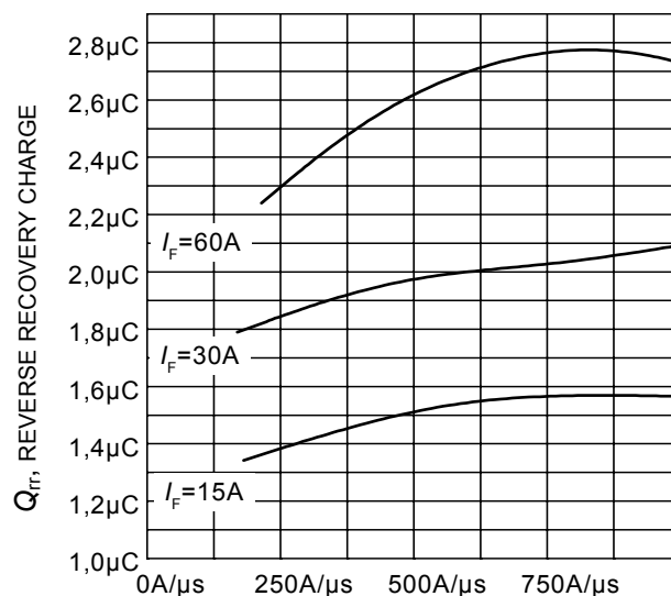
Figure 22. Typical reverse recovery charge as a function of diode current slope ( V_R=400V , T_J=150^{\circ}C , Dynamic test circuit in Figure E)
