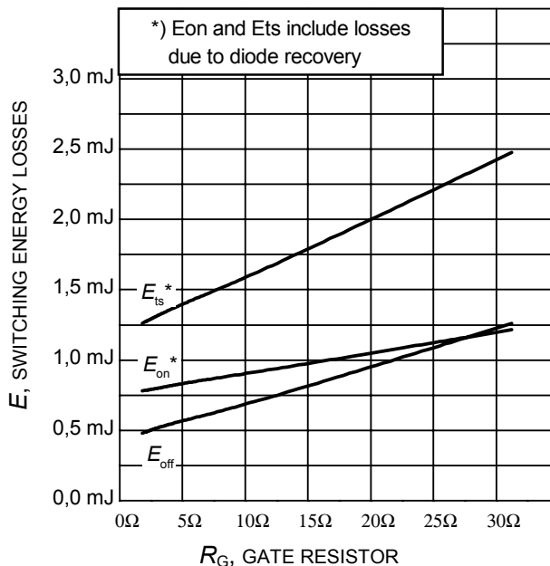
Figure 14. Typical switching energy losses as a function of gate resistor (inductive load, T_J=150^{\circ}\text{C} , V_{CE}=400\text{V} , V_{GE}=0/15\text{V} , I_C=30\text{A} , Dynamic test circuit in Figure E)
