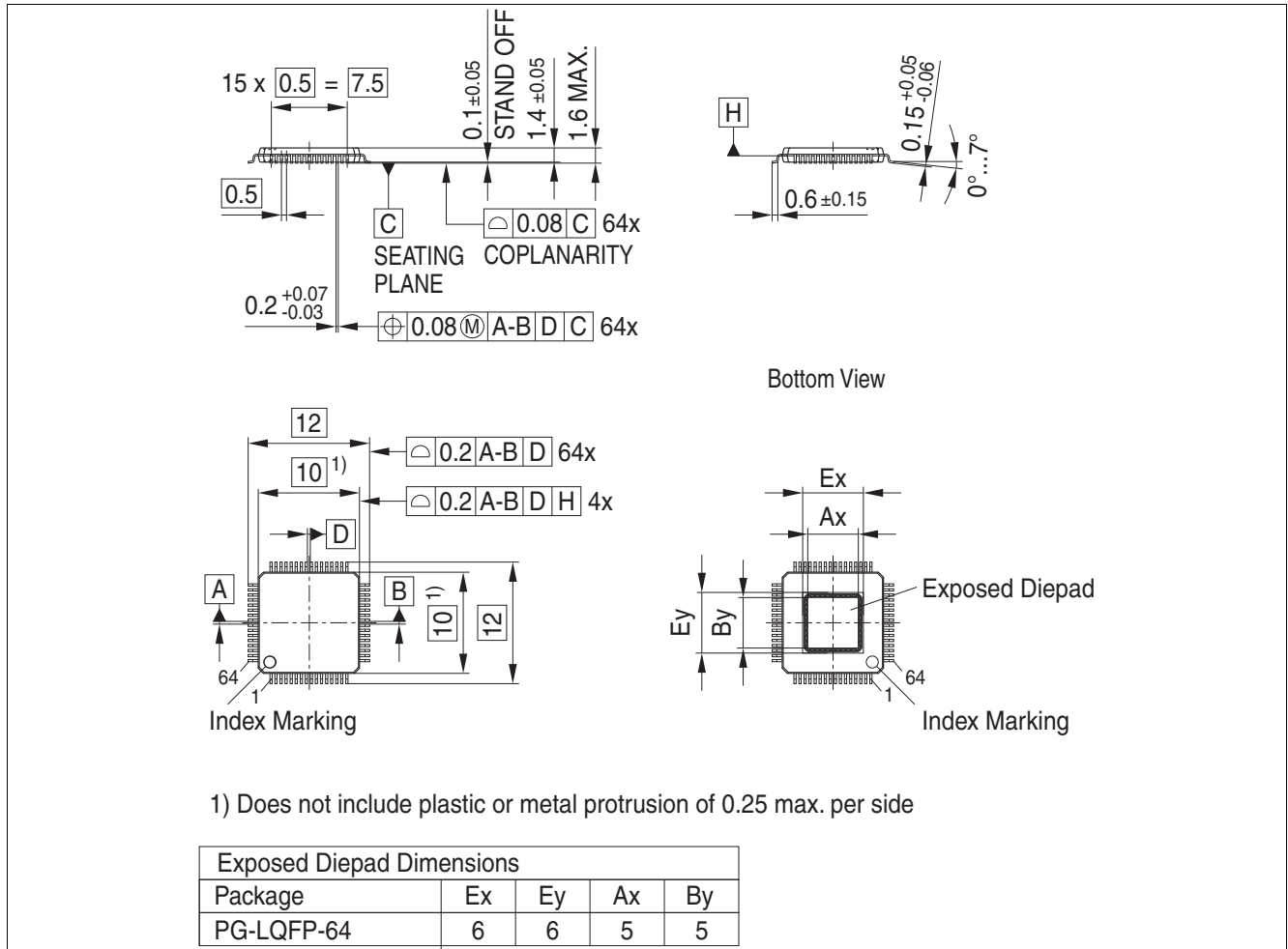
Figure 6 PG-LQFP-64
