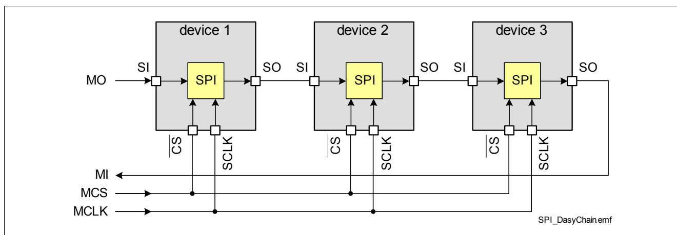
Figure 10 Daisy Chain Configuration
