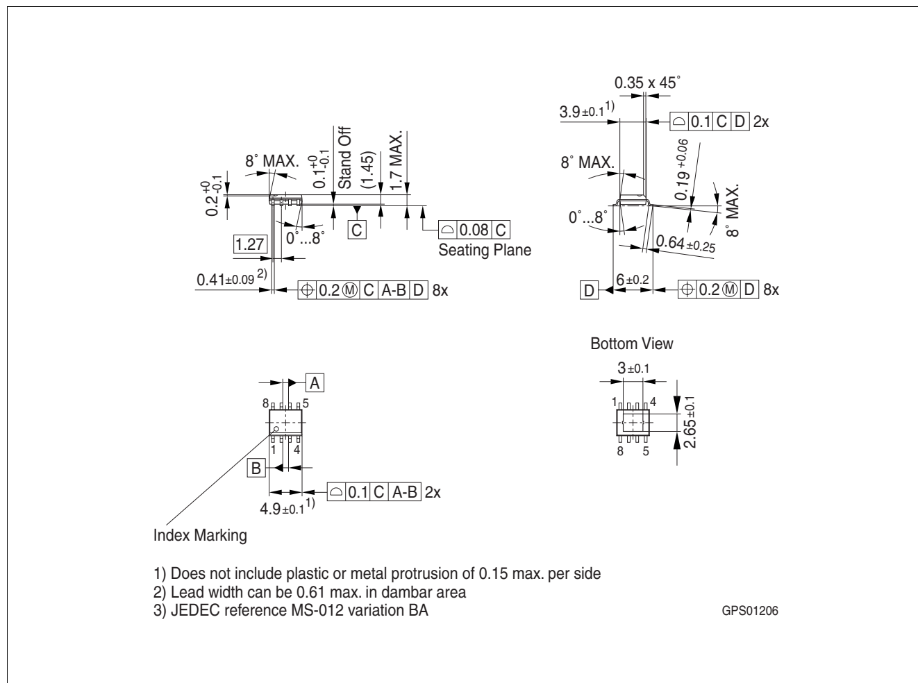
Figure 9 Outline PG-DSO-8
