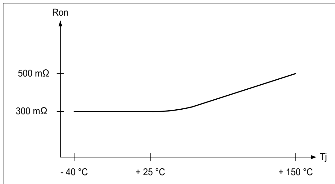
Figure 4 R_{on}
