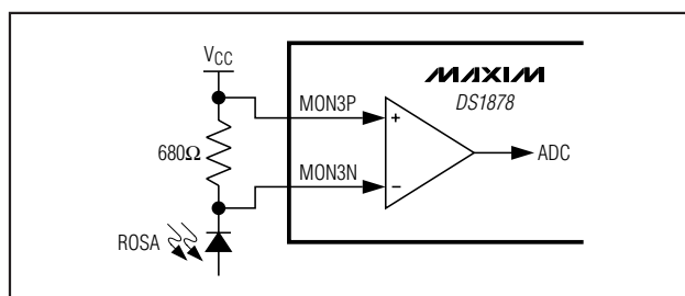
Figure 7. MON3 Differential Input for High-Side RSSI
