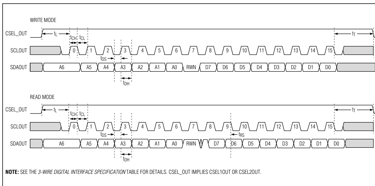
Figure 18. 3-Wire Timing
