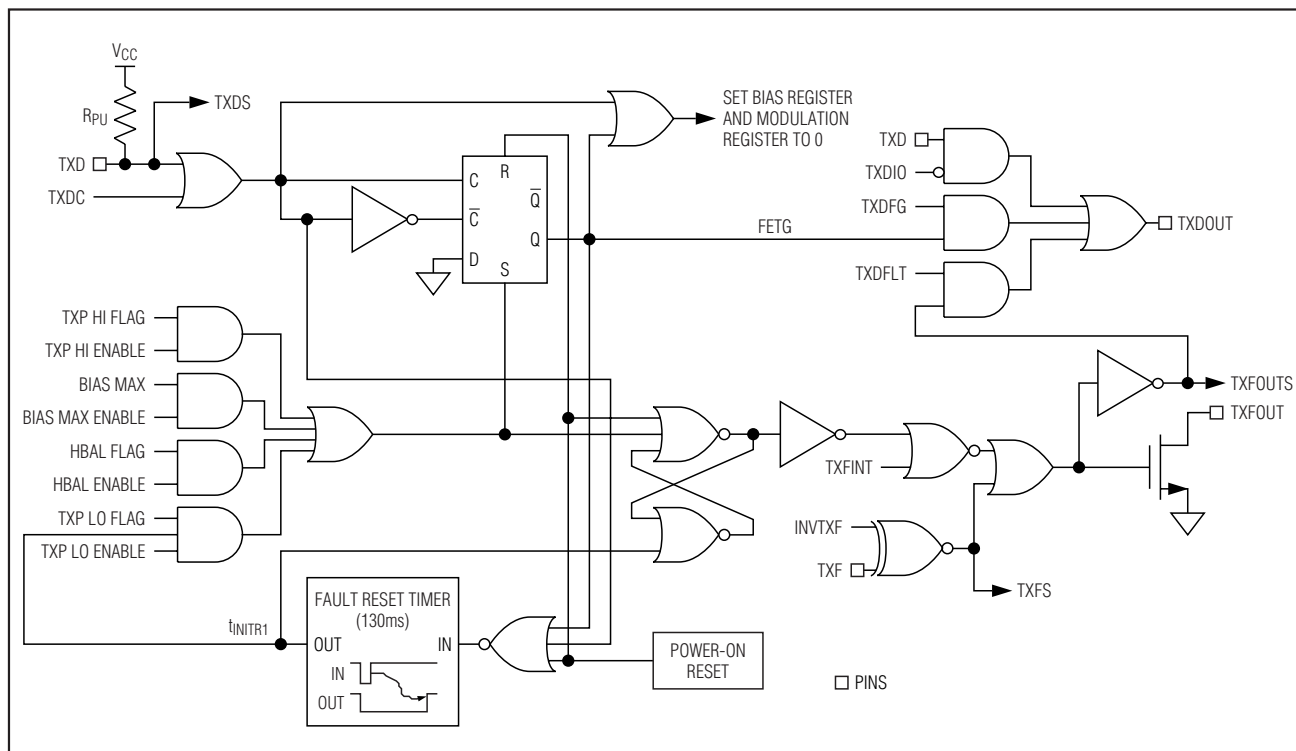
Figure 15. Logic Diagram 1
