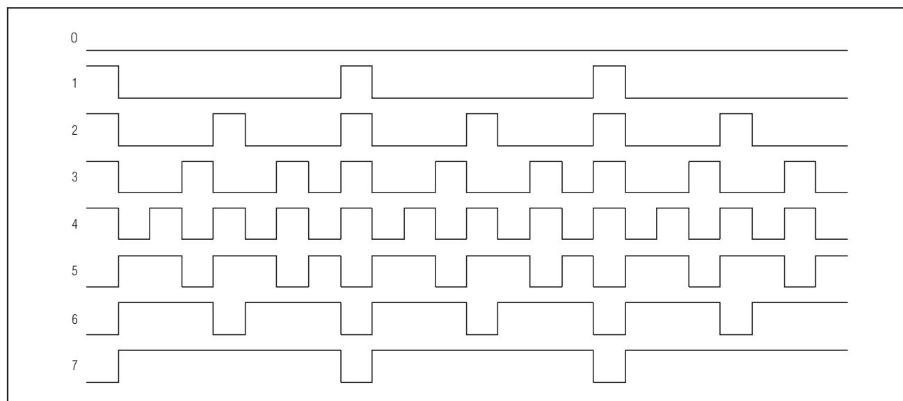
Figure 12. Delta-Sigma Outputs
