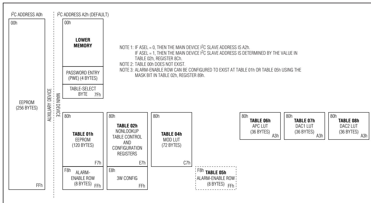
Figure 22. Memory Map
