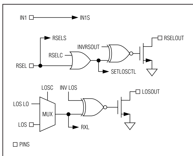
Figure 16. Logic Diagram 2
