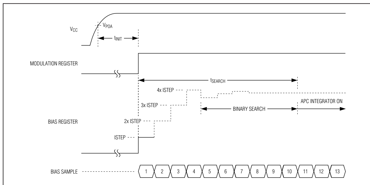
Figure 2. Power-Up Timing
