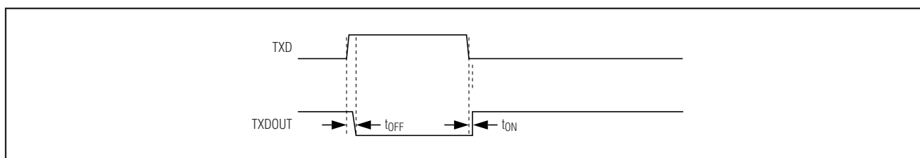
Figure 3. TXD Timing
