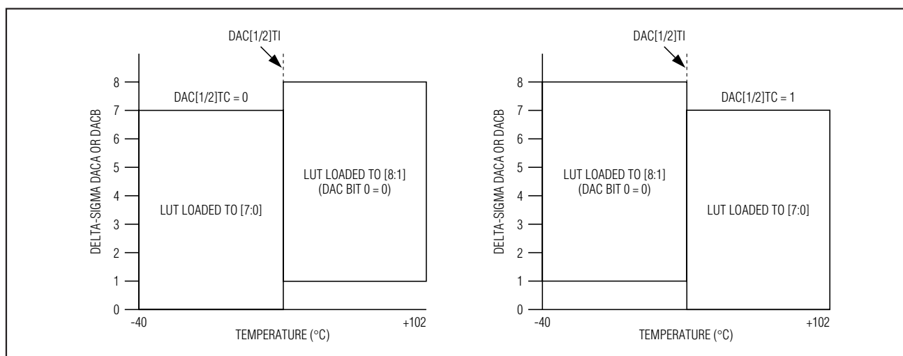
Figure 13. DAC1/DAC2 LUT Assignments
