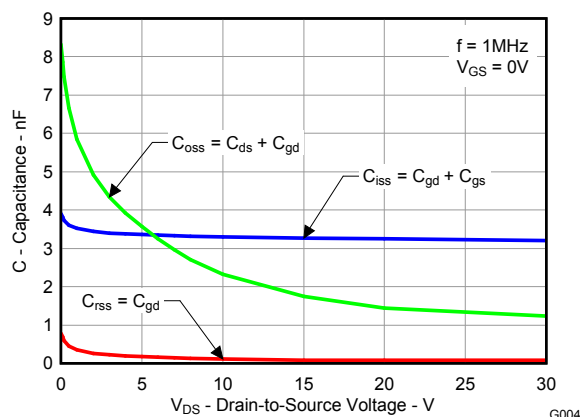
Figure 5. Capacitance
