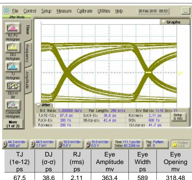
Figure 21. Test Point 2
