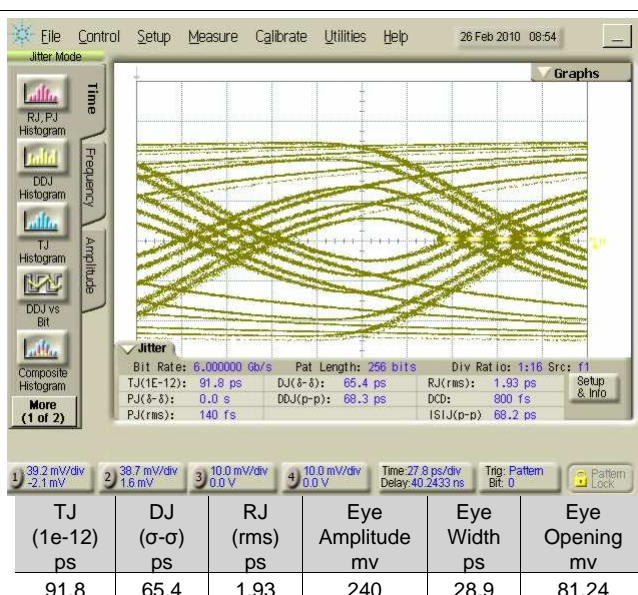
Figure 11. Test Point 2
