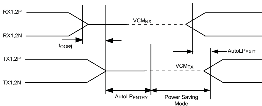
Figure 4. Auto Low-Power Mode Enter and Exit Timing
