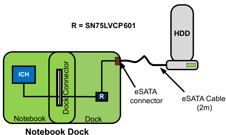
Figure 26. Typical SN75LVCP601 Placement in the System
