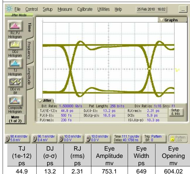
Figure 22. Test Point 3
