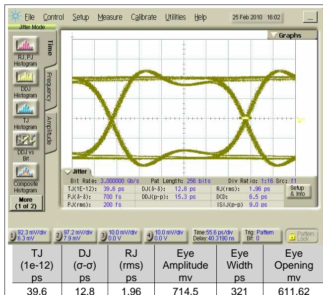
Figure 17. Test Point 3
