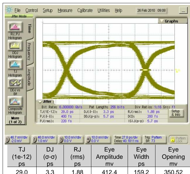
Figure 10. Test Point 1
