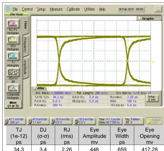
Figure 20. Test Point 1
