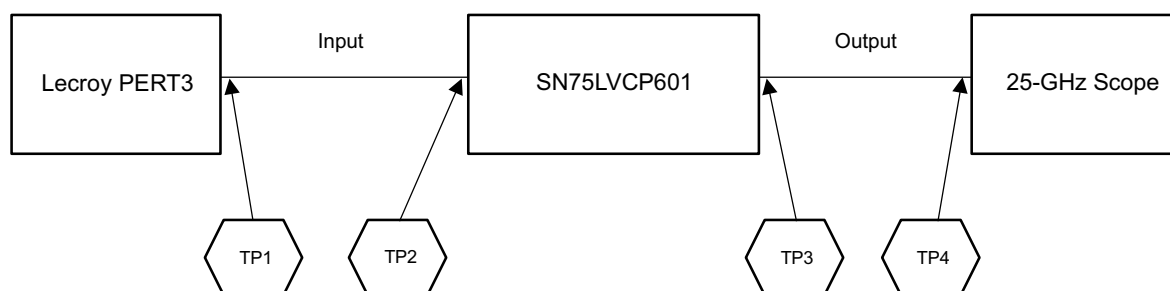
Figure 28. Measurement Set-up
