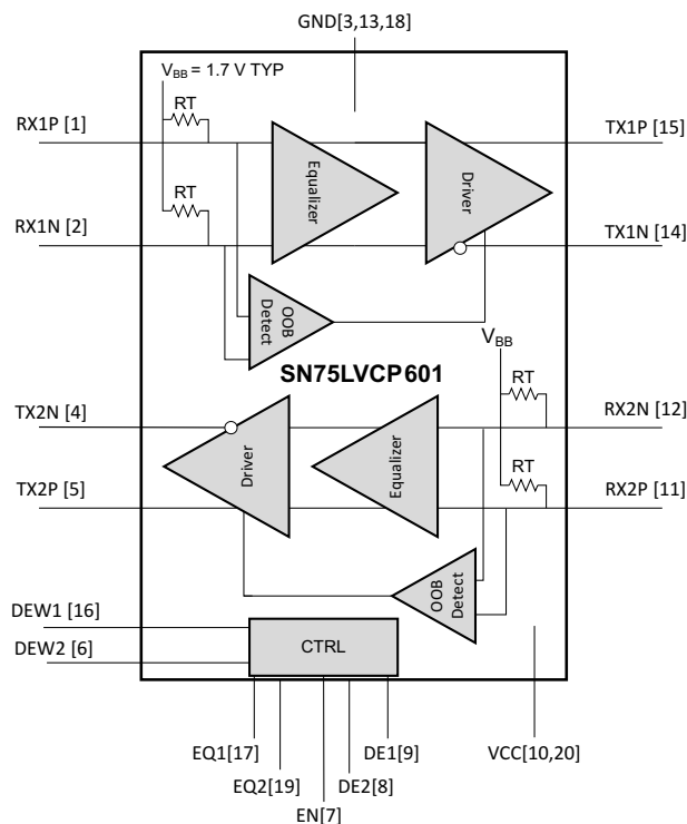
Figure 25. Data Flow Block Diagram
