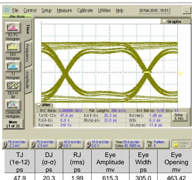
Figure 18. Test Point 4 With LVCP601
