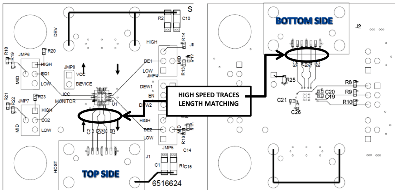
Figure 47. SN65LVCP601 EVM
