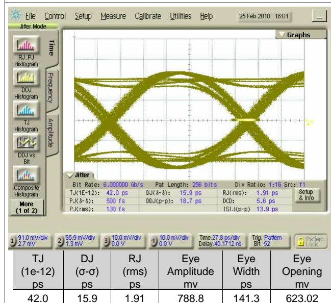
Figure 12. Test Point 3
