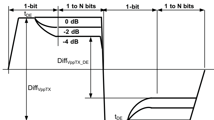
Figure 5. TX Differential Output
