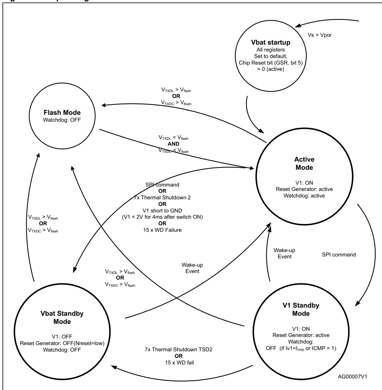
Figure 8. Operating modes
