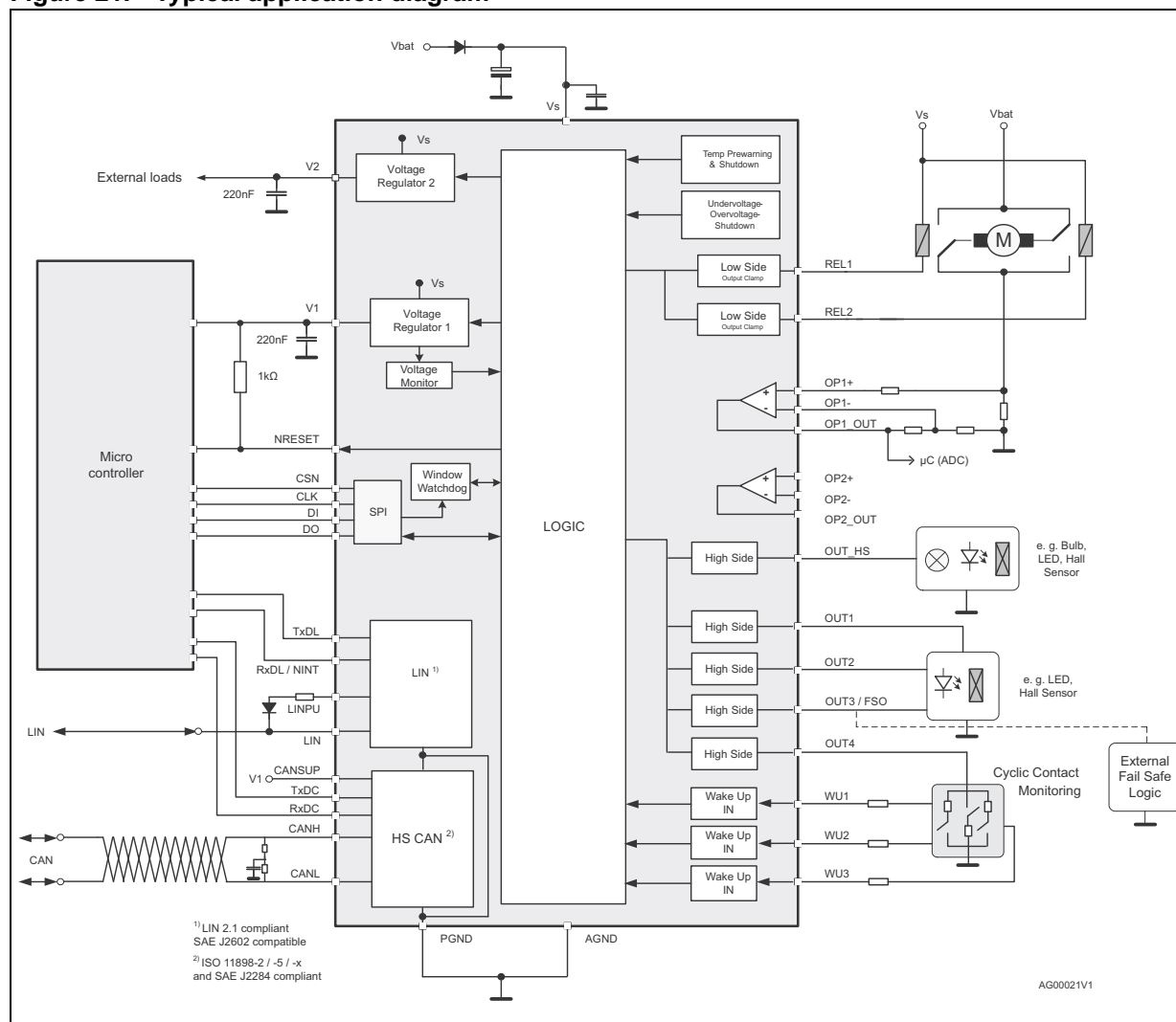
Figure 21. Typical application diagram
