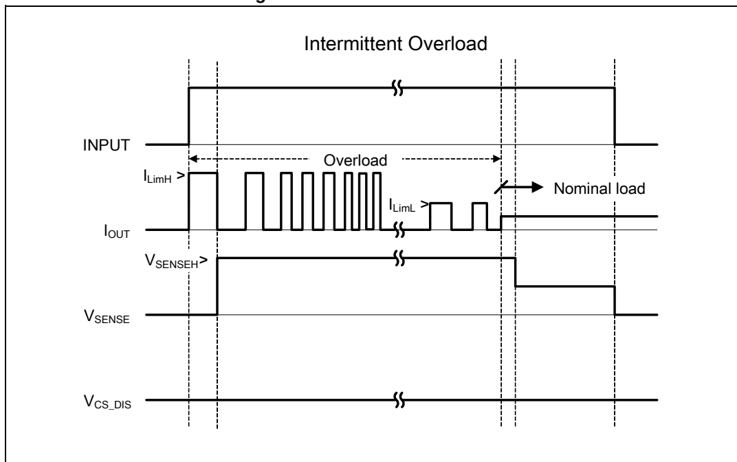
Figure 12. Intermittent overload
