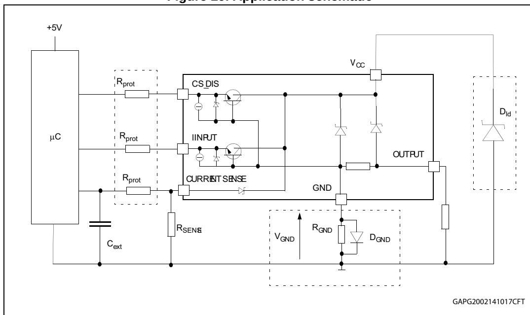
Figure 29. Application schematic
