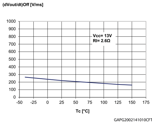
Figure 25. Turn-off voltage slope
