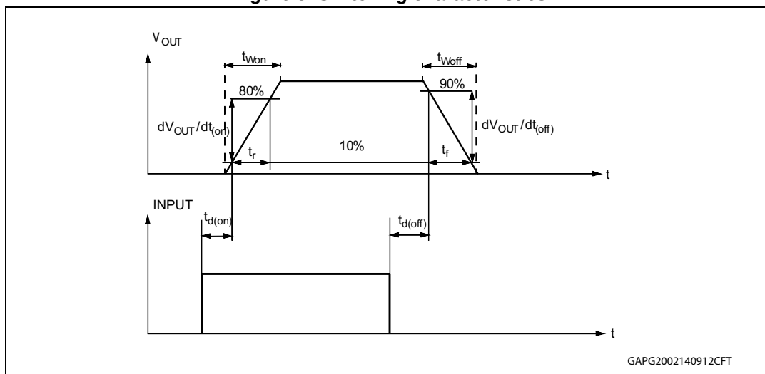
Figure 5. Switching characteristics
