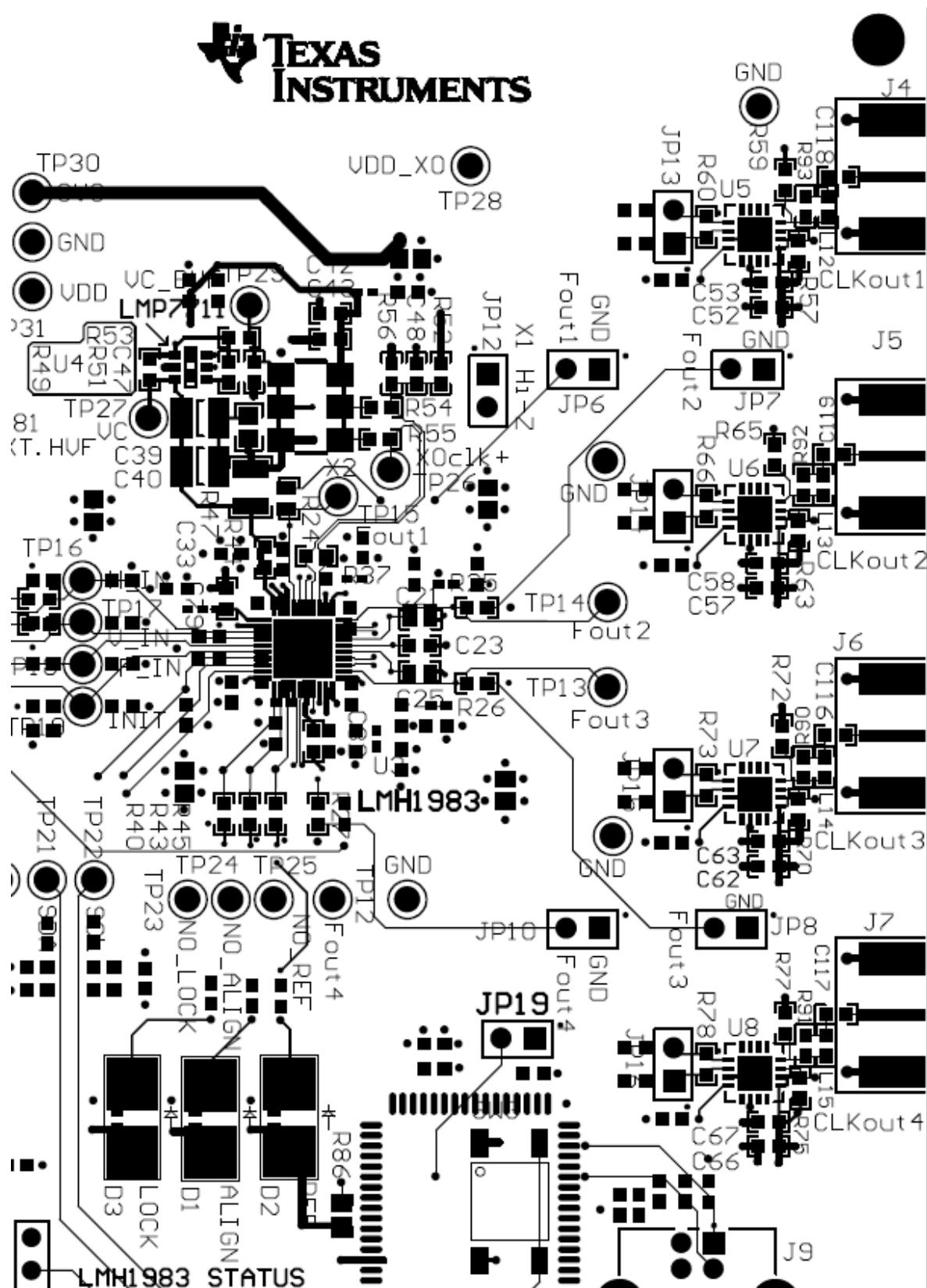
Figure 36. LMH1983 Example Layout
