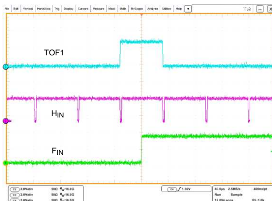
Figure 14. TOF1 Timing
