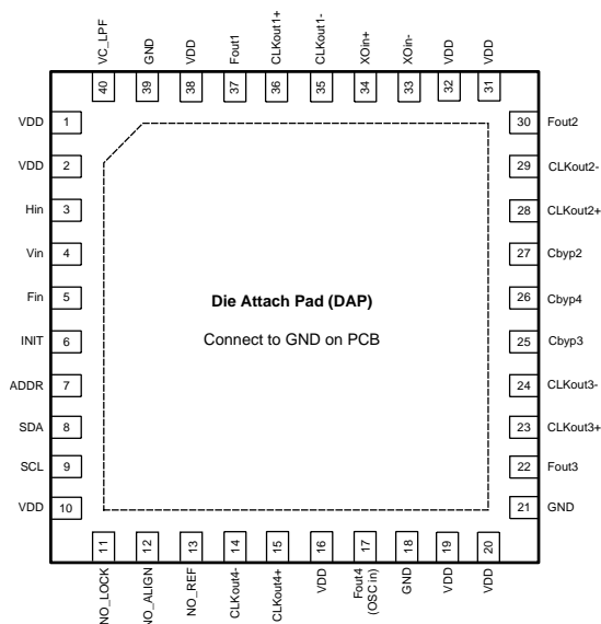
Pin Functions
