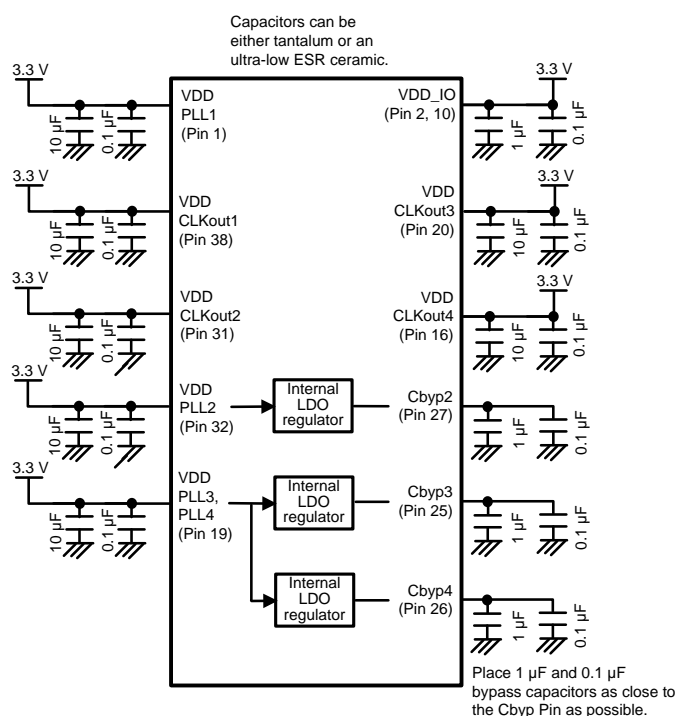
Figure 32. LMH1983 Power Supply Connection Diagram
