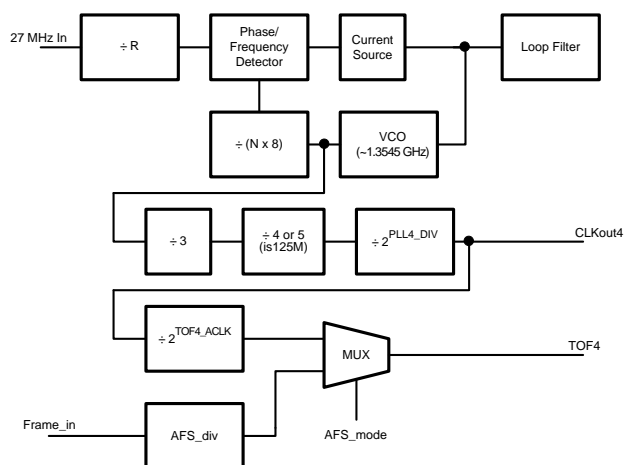
Figure 12. PLL4 Block Diagram
