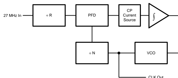
Figure 11. PLL2 / PLL3 Block Diagram
