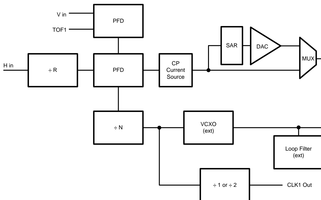
Figure 9. PLL1 Block Diagram
