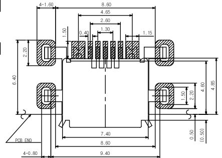
USB-IF REVERSE type Pattern USB-IF Recommended RIVERSE type Pattern (Tolerance : \pm 0.05 )
