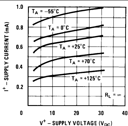
Figure 1. Supply Current
