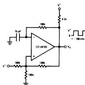
Figure 15. Driving CMOS
