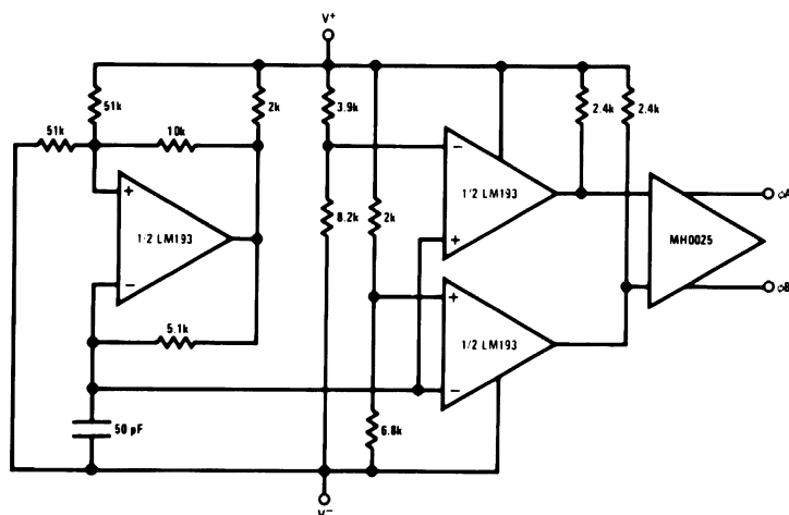
Figure 14. MOS Clock Driver
