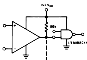
Figure 15. Driving CMOS
