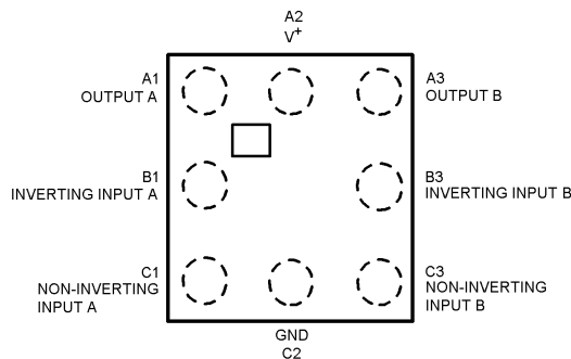
8-Pin DSBGA YZR Package Top View
