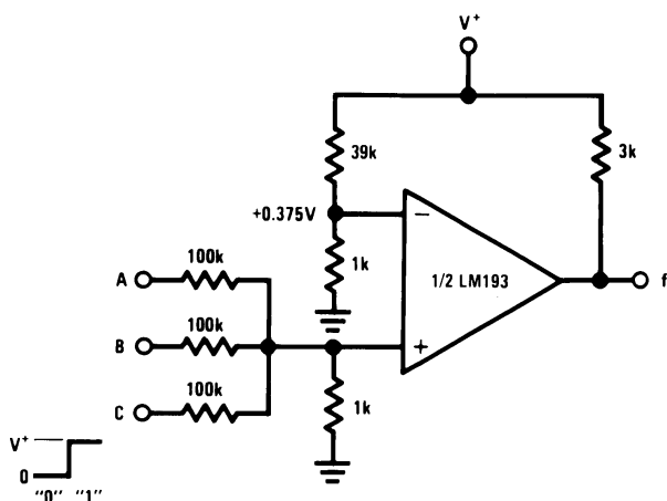
Figure 25. And Gate
