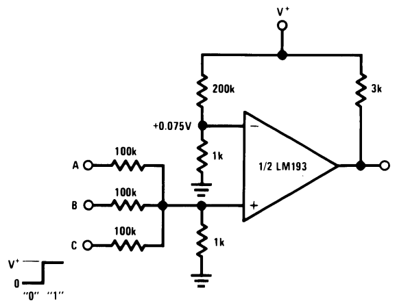
Figure 26. Or Gate
