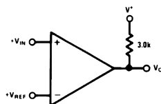
Figure 12. Basic Comparator
