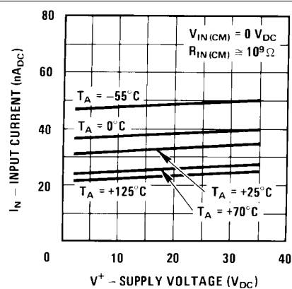
Figure 2. Input Current
