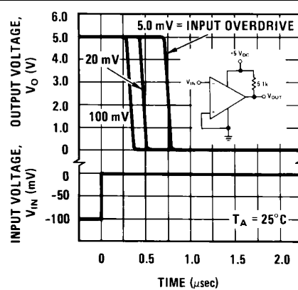
Figure 4. Response Time for Various Input Overdrives—Negative Transition
