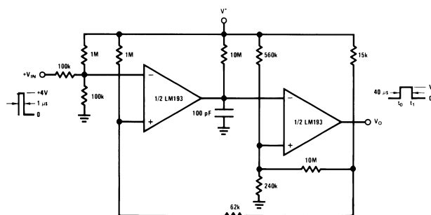
Figure 34. One-Shot Multivibrator With Input Lock Out
