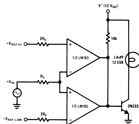
Figure 26. Or Gate
