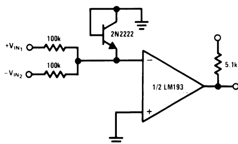
Figure 27. Large Fan-In and Gate
