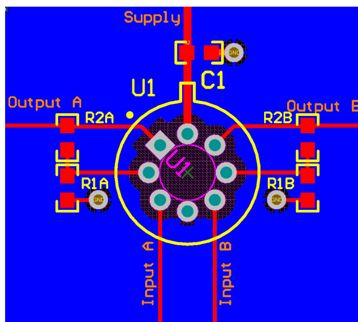
Figure 38. Layout Example
