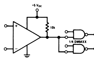
Figure 16. Driving TTL
