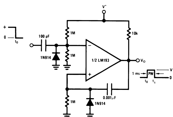
Figure 32. One-Shot Multivibrator
