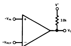
Figure 11. Basic Comparator
