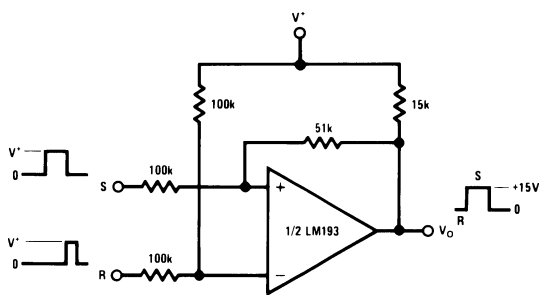
Figure 33. Bi-Stable Multivibrator
