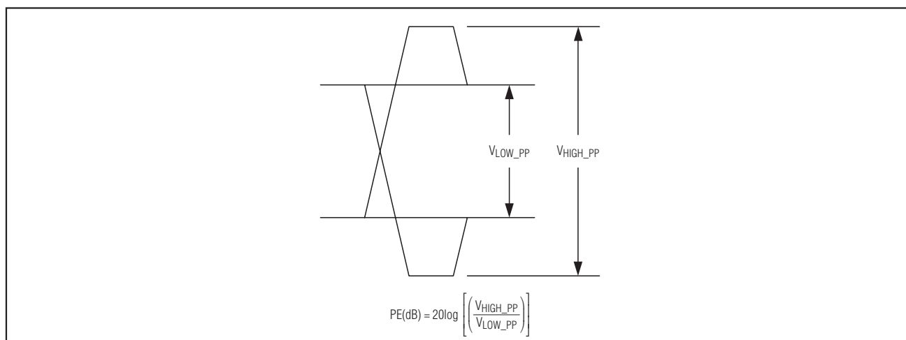
Figure 1. Output Preemphasis
