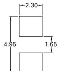
Recommended Pad Layout
