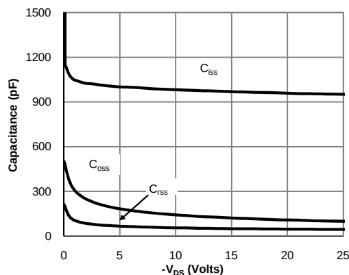
Figure 8: Capacitance Characteristics
