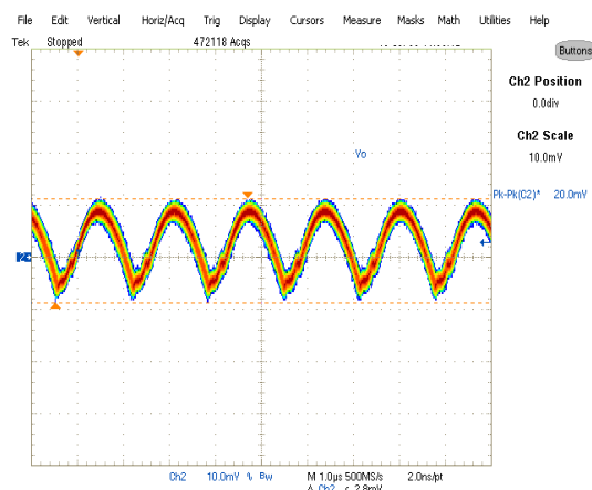
Fig. 20: Output Voltage Ripple, 12A load Ch2: V_o
