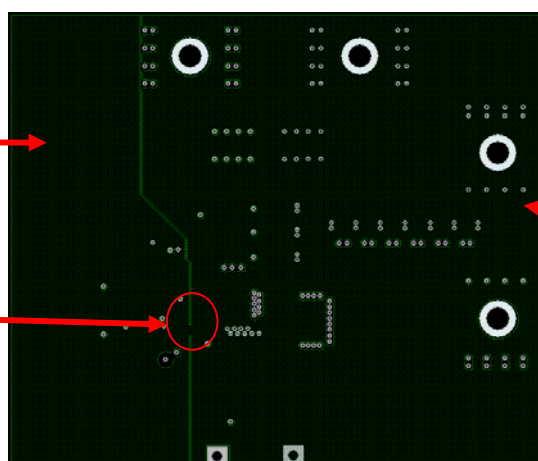
Fig.26c. IRDC3841W demoboard layout considerations – Mid Layer 1
