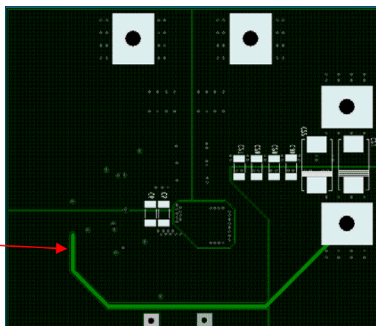
Fig.26b. IRDC3841W demoboard layout considerations – Bottom Layer
