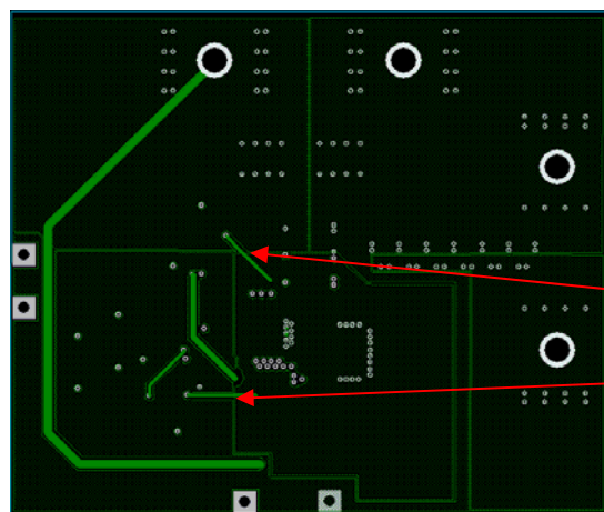
Fig.26d. IRDC3841W demoboard layout considerations – Mid Layer 2
