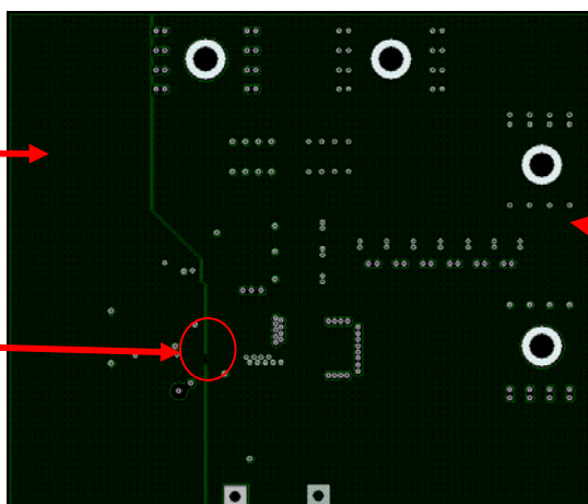
Fig. 26c. IRDC3843A demoboard layout considerations – Mid Layer 1
