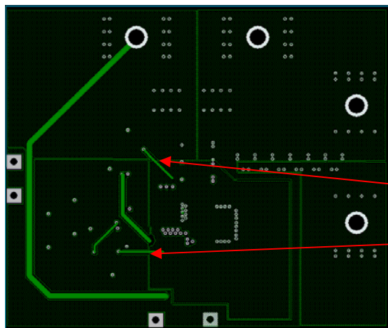
Fig. 26d. IRDC3843A demoboard layout considerations – Mid Layer 2
