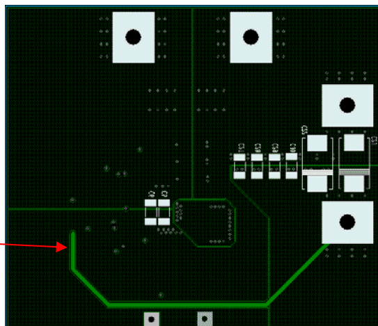
Fig. 26b. IRDC3843A demoboard layout considerations – Bottom Layer
