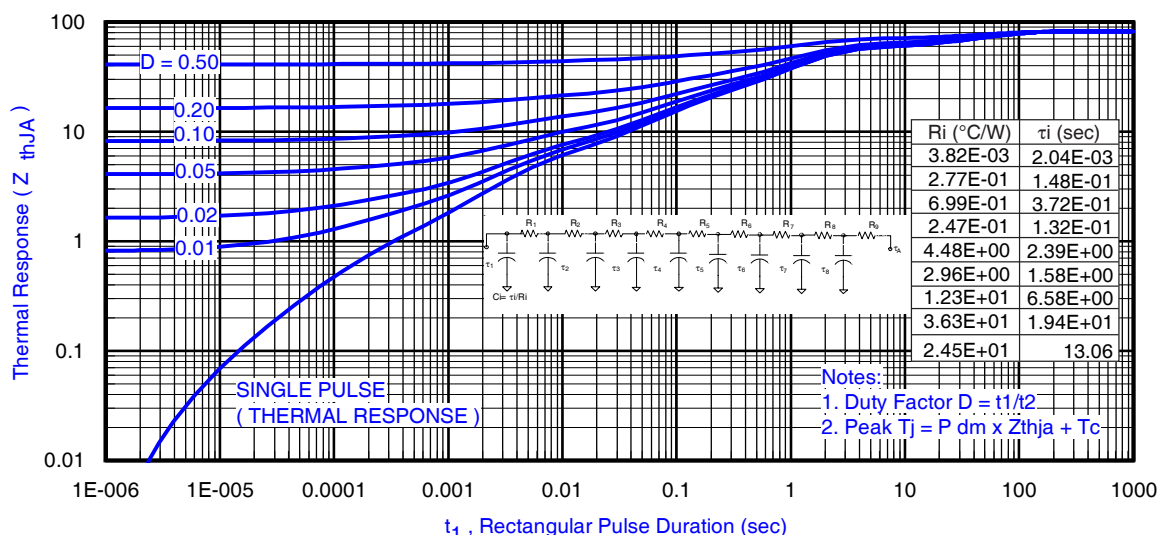
Fig 3. Maximum Effective Transient Thermal Impedance, Junction-to-Ambient ⑩ (At lower pulse widths Z_{thJA} & Z_{thJC} are combined)
