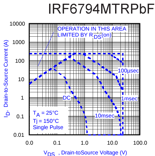
Fig 11. Maximum Safe Operating Area
