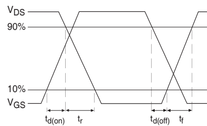
Fig 19b. Switching Time Waveforms
