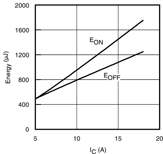
Fig. 12 - Typ. Energy Loss vs. I_C T_J = 175^{\circ}\text{C} ; L = 1000\mu\text{H} ; V_{CE} = 600\text{V} ; R_G = 22\Omega ; V_{GE} = 15\text{V}
