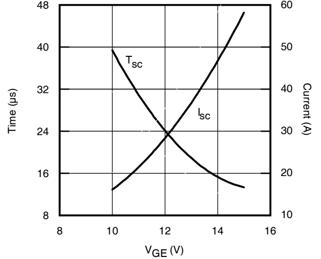
Fig. 16 - V_{GE} vs. Short Circuit Time
