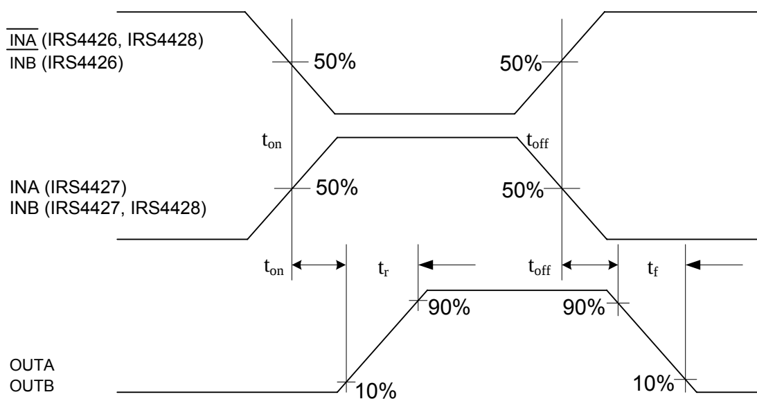
Figure 2: Switching Time Waveform Definitions
