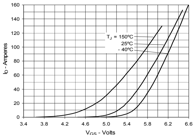
Fig. 7. Input Admittance
