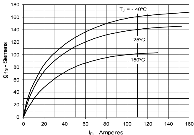
Fig. 8. Transconductance
