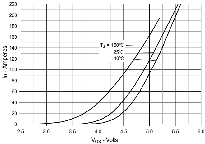
Fig. 7. Input Admittance
