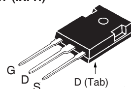
TO-247 (IXFH)
