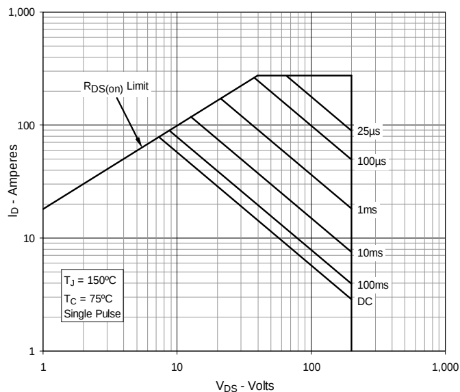
Fig. 14. Forward-Bias Safe Operating Area
