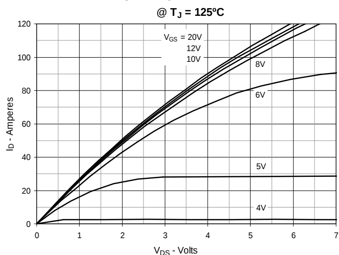
Fig. 3. Output Characteristics
