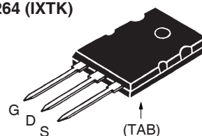
TO-264 (IXTK)
