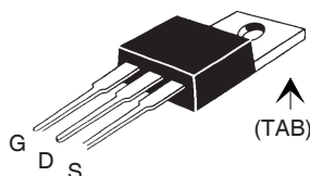
TO-220 (IXTP)
