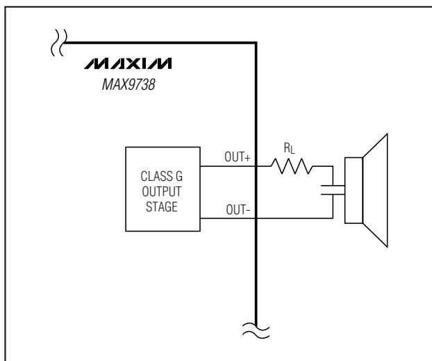
Figure 3. Driving a Ceramic Speaker
