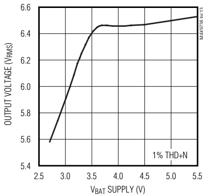
MAXIMUM OUTPUT VOLTAGE vs. VBAT SUPPLY
