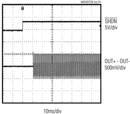
STARTUP WAVEFORM
