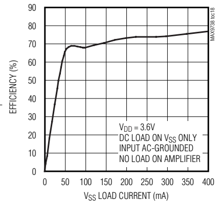
EFFICIENCY vs. VSS LOAD CURRENT
