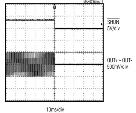
SHUTDOWN WAVEFORM
