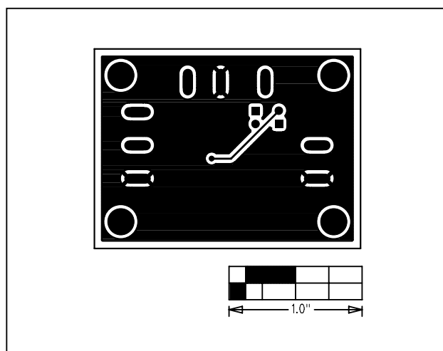
Figure 5. MAXFILTERBRD PCB Layout—Solder Side
