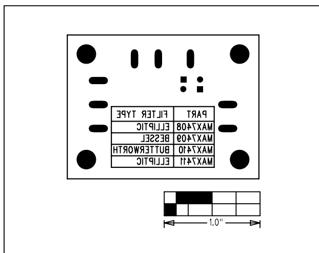
Figure 6. MAXFILTERBRD Component Placement Guide—Solder Side
