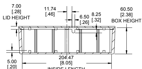
SECTION A-A SIDE VIEW
