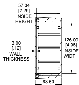
SECTION B-B END VIEW
