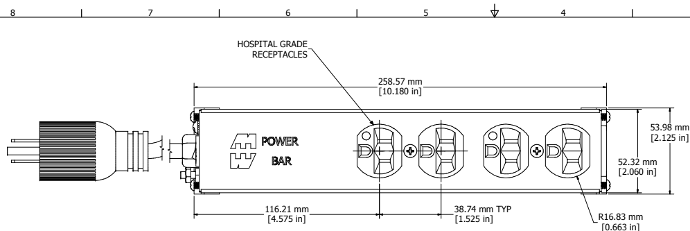
ASSEMBLY - VIEW FROM TOP
