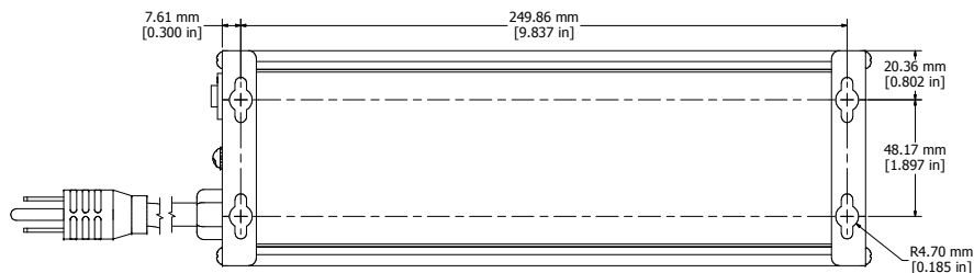
ASSEMBLY - VIEW FROM BOTTOM
