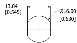
PANEL CUTOUT (NOT TO SCALE)
