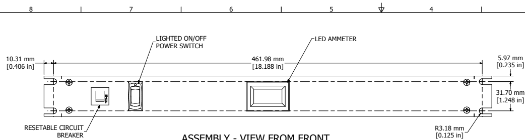
ASSEMBLY - VIEW FROM FRONT
