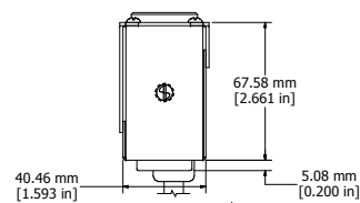
ASSEMBLY - VIEW FROM SIDE
