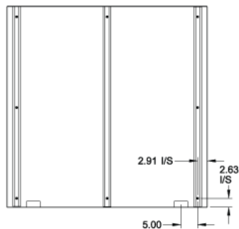
Stiffener Layout
