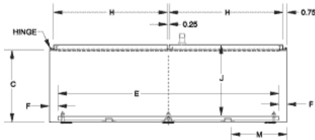
Section Y-Y
