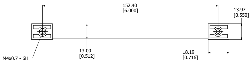
BOTTOM VIEW
