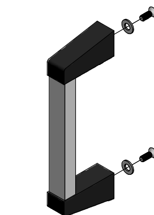
EXPLODED HANDLE ASSEMBLY
