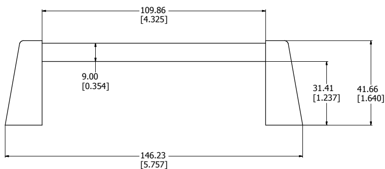
SIDE VIEW
