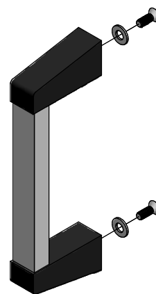
EXPLODED HANDLE ASSEMBLY
