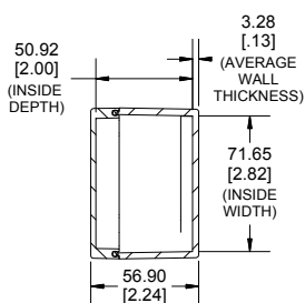
SECTION A-A END VIEW
