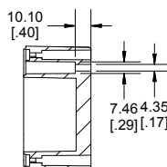
SECTION C-C MOUNTING HOLE
