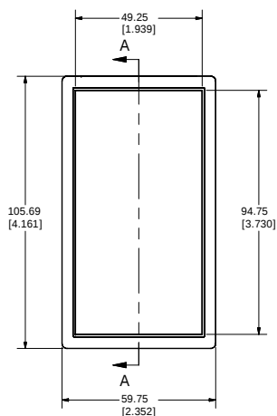
Top View of Assembly
