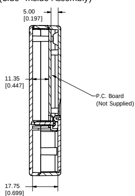
SECTION A-A (Side Inside Assembly)
