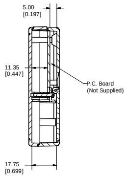
SECTION E-E (Side Inside Assembly)
