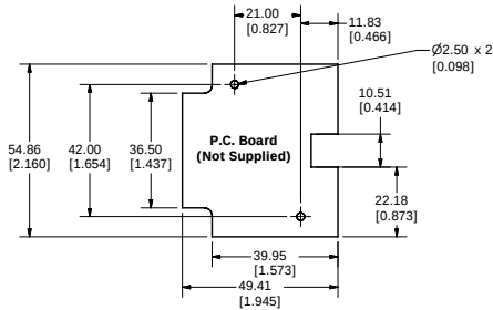
Maximum P.C. Board Size
