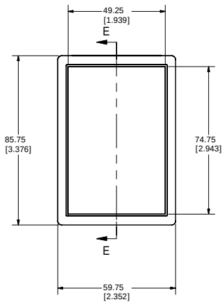
Top View of Assembly
