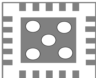
FIGURE 8. EXPOSED PAD
