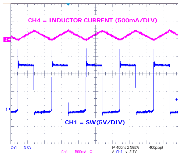
FIGURE 2. PWM WAVEFORM IN TRICKLE MODE
