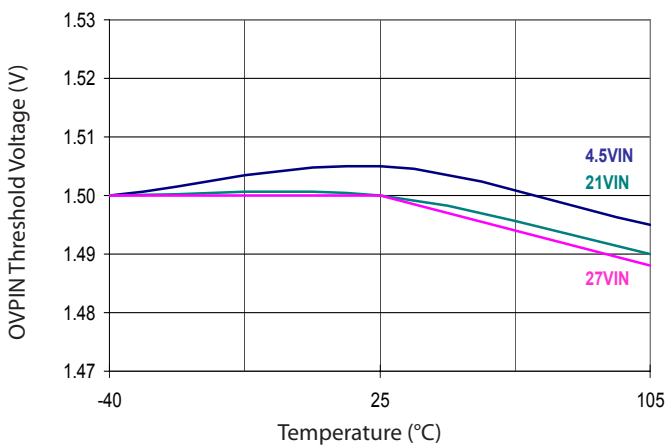
OVPIN Threshold vs. Temperature
