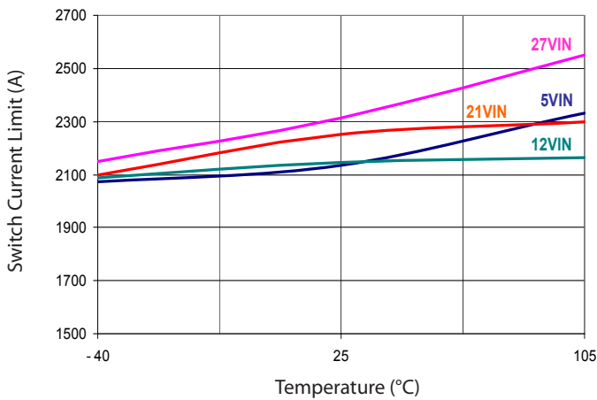
Switch Current Limit vs. Temperature
