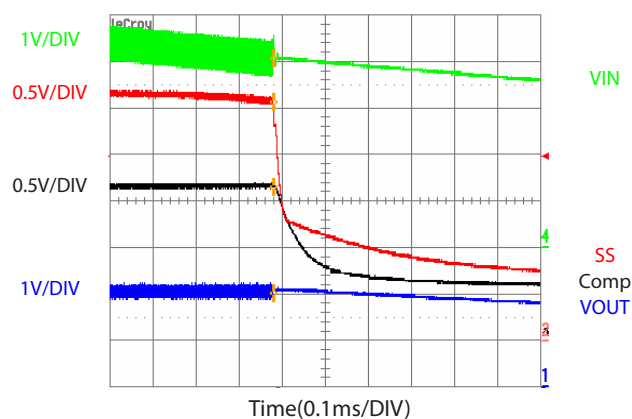
Shutdown by Vin
