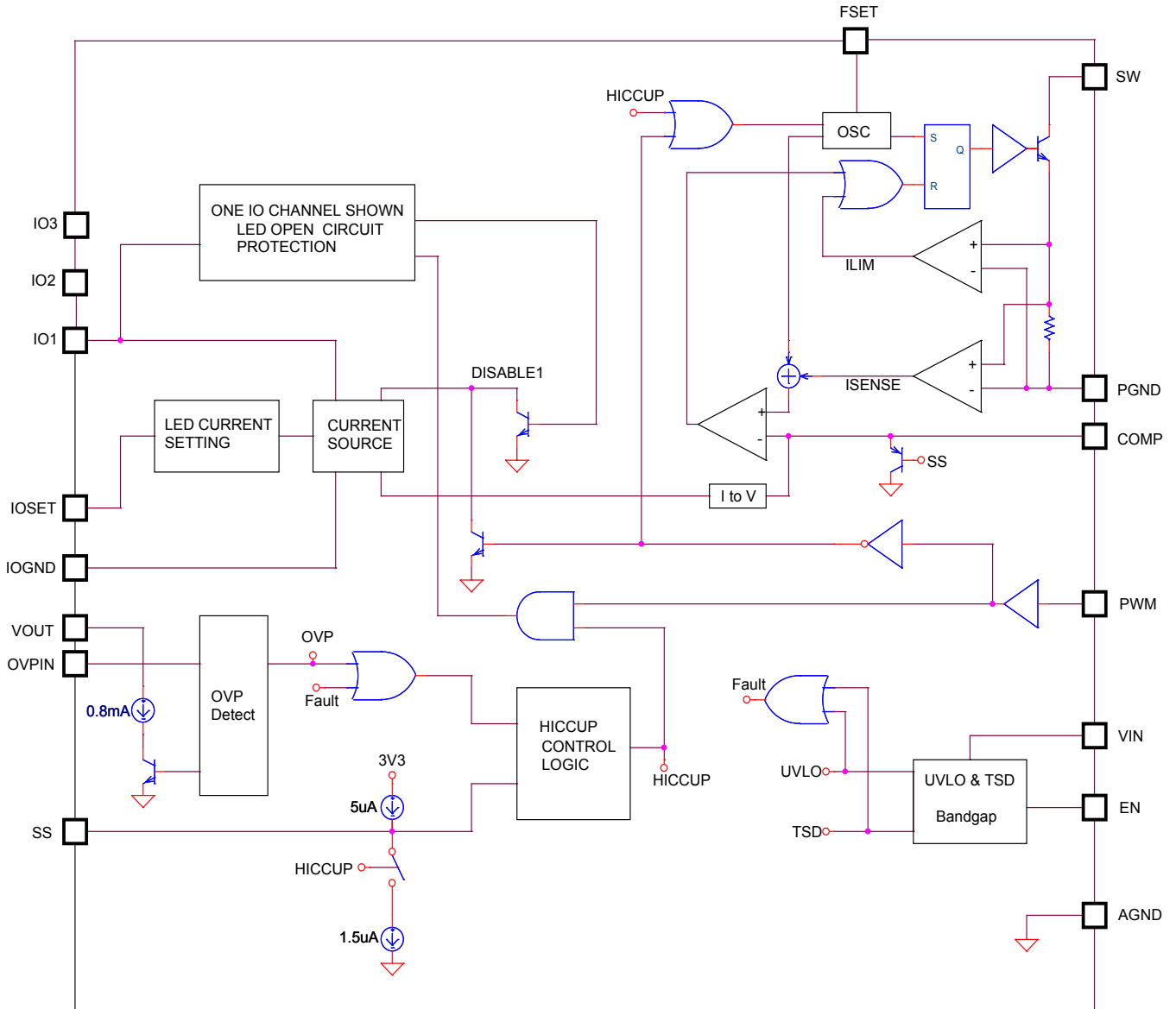
Figure 1. SC443 Block Diagram
