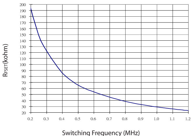
Switching frequency setting
