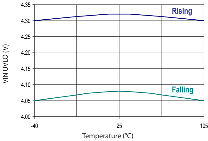
UVLO Threshold vs. Temperature
