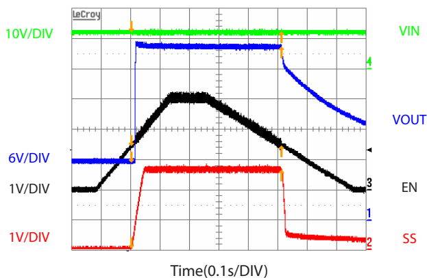
Start up and Shutdown by EN
