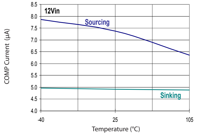
COMP Current vs. Temperature
