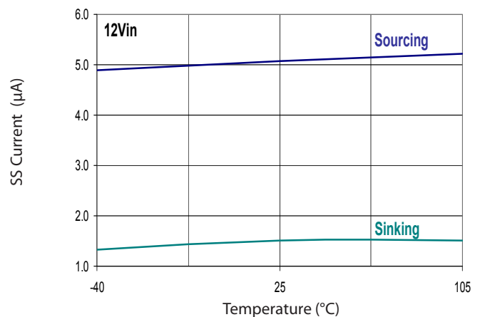
SS Current vs. Temperature
