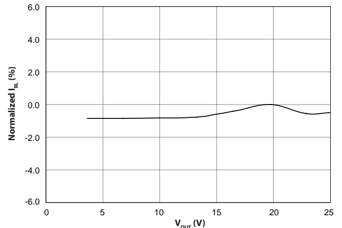
Normalized I_{BL} vs. Output Voltage
