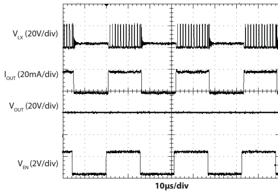
PWM Operation at 32kHz and 50% Duty Cycle
