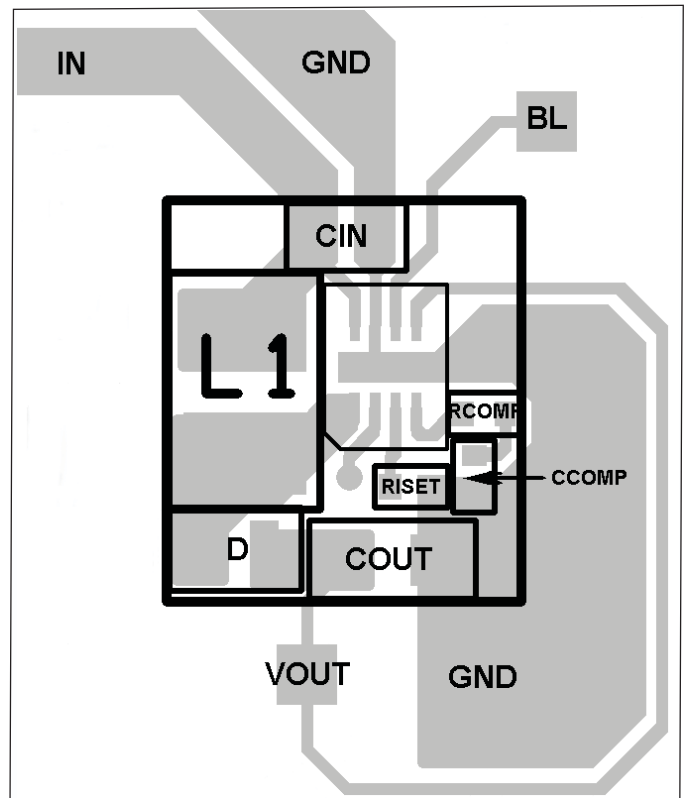
Figure 2– Layout
