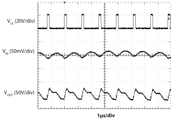
Typical Waveforms at V_{IN} = 3.6V
