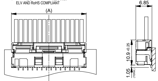
嵌合図 MATED CONNECTOR (SCALE : 2:1)
